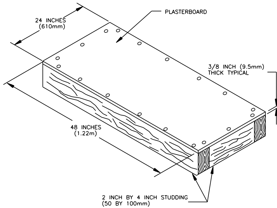
Figure 173.1 Test wall
