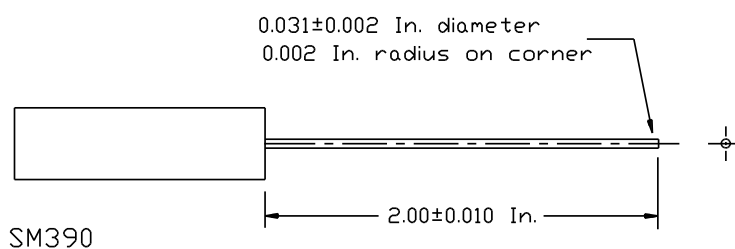
Figure 139.1 Small test probe
