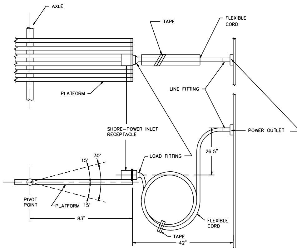
Figure SB10.1 Mechanical strength test apparatus
