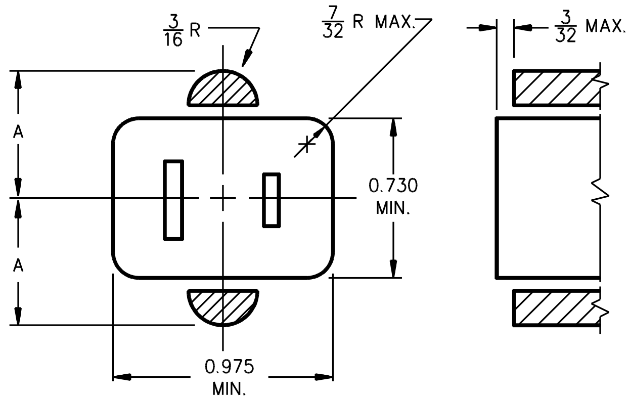
Figure 23.3 Minimum outlet face dimensions
