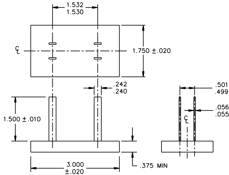
Figure 124.3 Pushout tool
