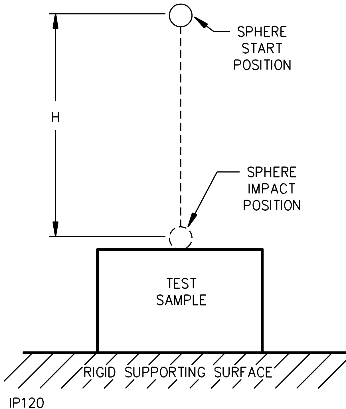
Figure 140.3 Vertical-ball impact test
