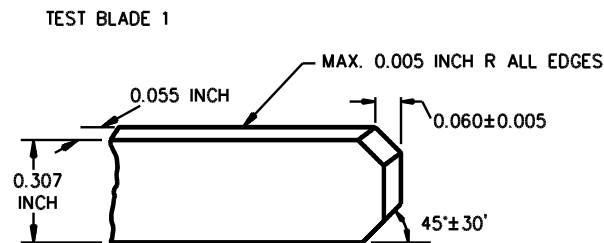
Figure 100.1 Improper insertion test blades
