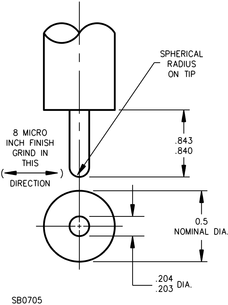
Figure SC13.2 Oversize grounding pin
