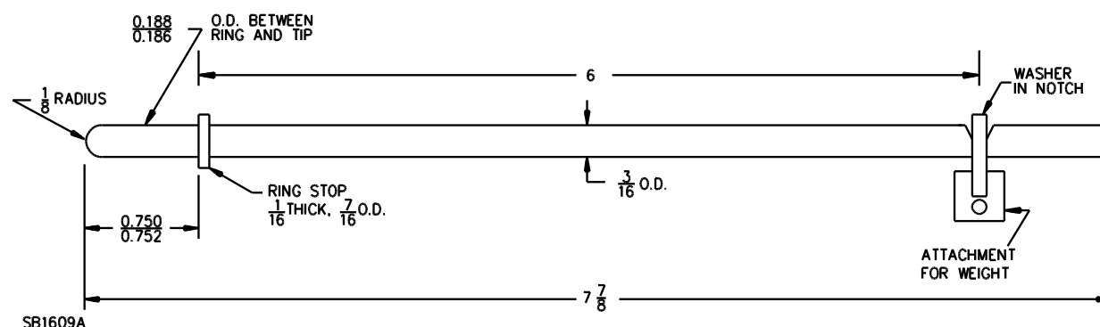
Figure 125.1 Test pin A
