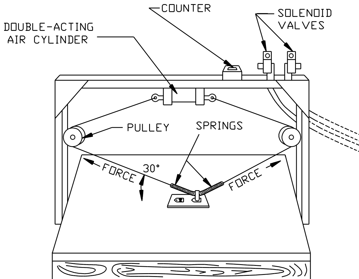
Figure 173.2 Wall mounting secureness test
