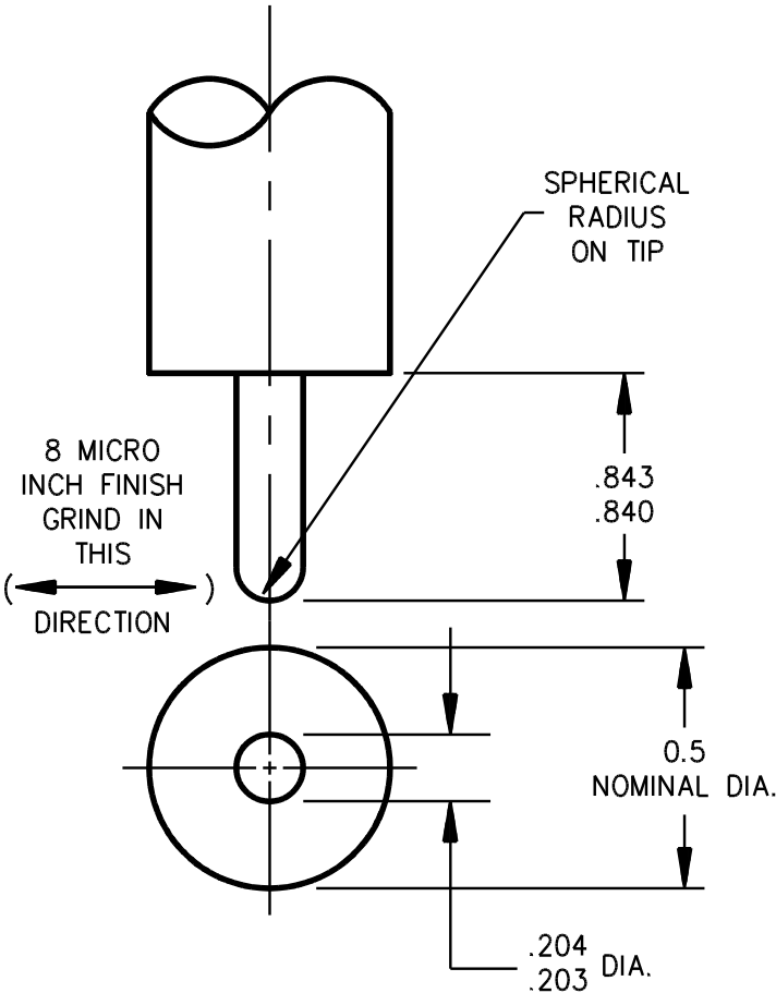
Figure SC25.1 Oversize grounding pin
