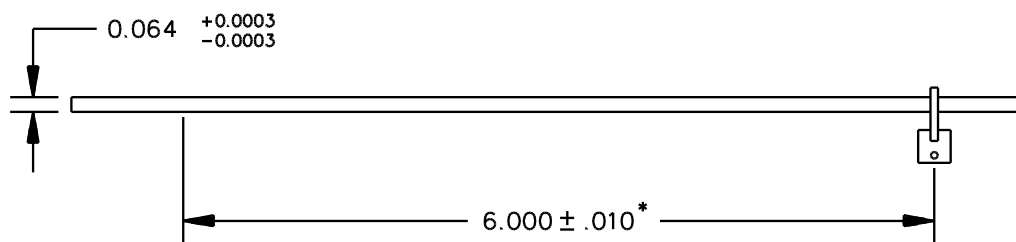
Figure 136.2 14 AWG test pin
