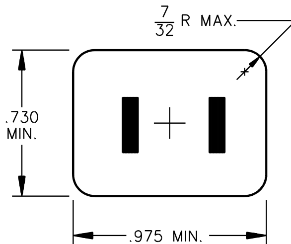
Figure 17.1 Minimum attachment plug face dimensions
