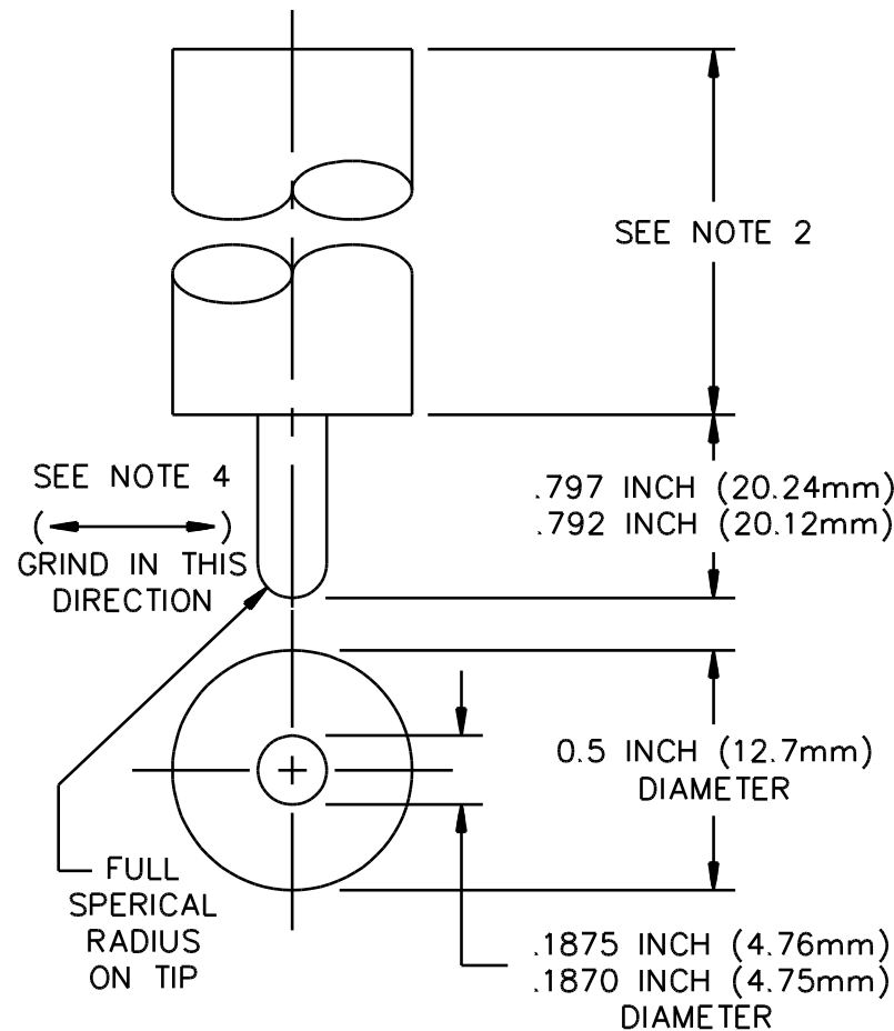
Figure 125.4 4 oz (113 g) ground pin
