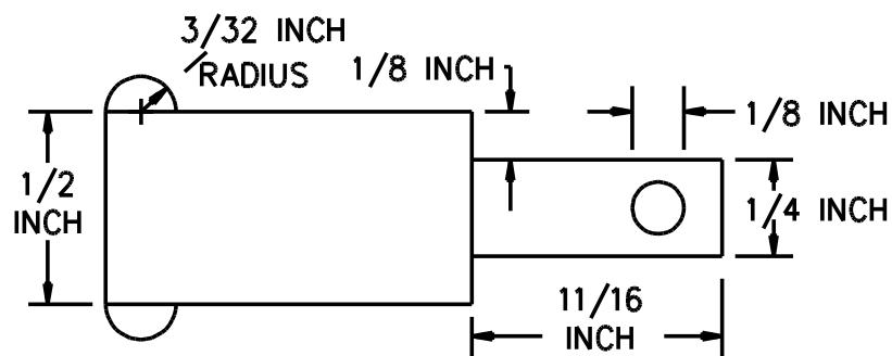
Figure 74.1 Reference plug
