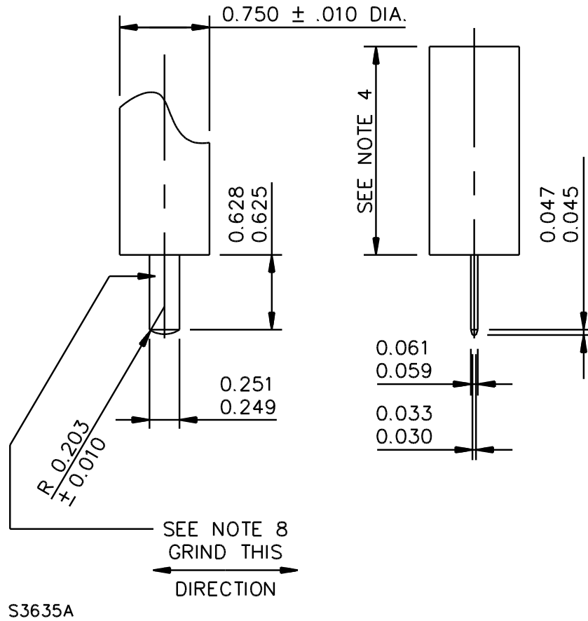
Figure 111.2 Test blade
