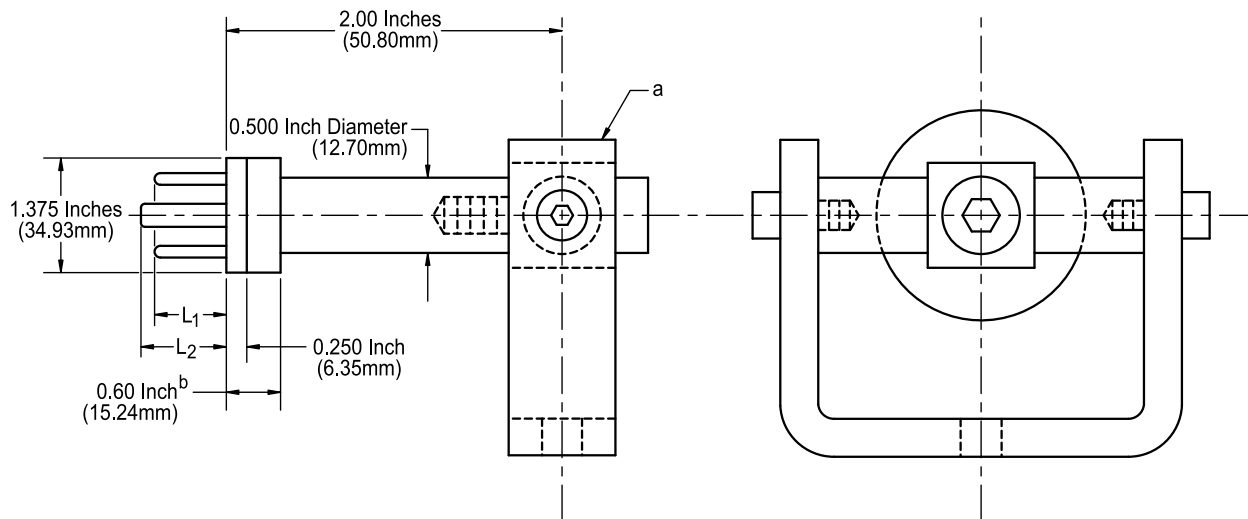
Figure SC21.2 Typical test plug for abrupt plug removals
