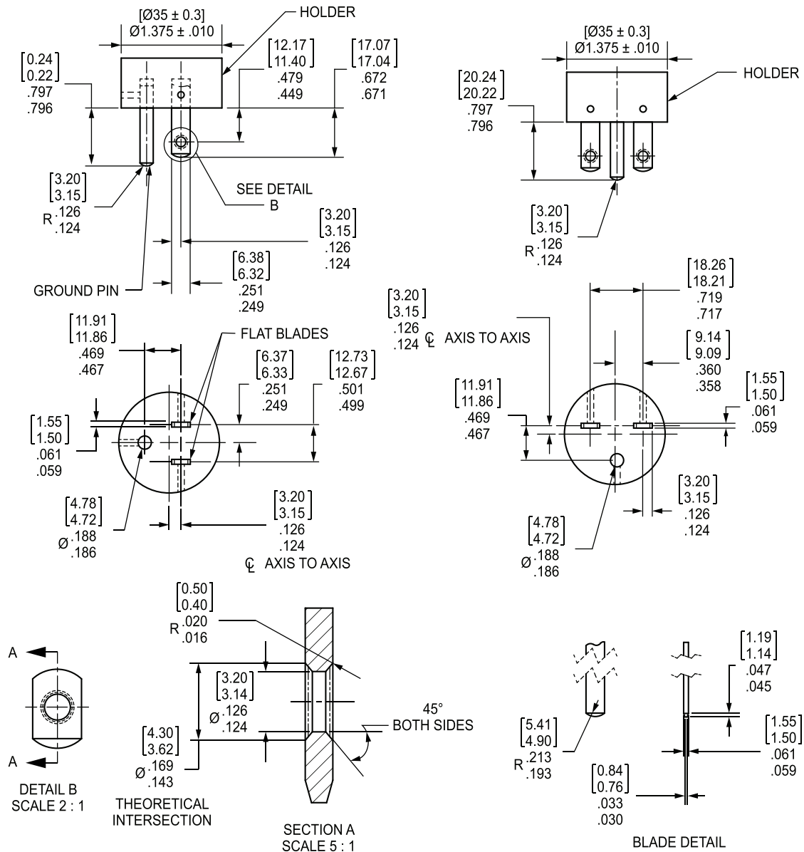
Figure 111.1 Test gauge
