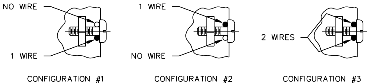
Figure 123.1 Wiring configurations for back-wired terminals
