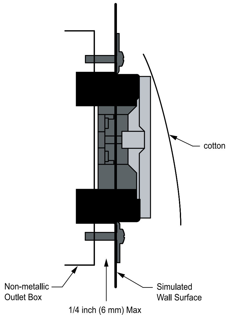
Figure 143.1 Receptacle installation
