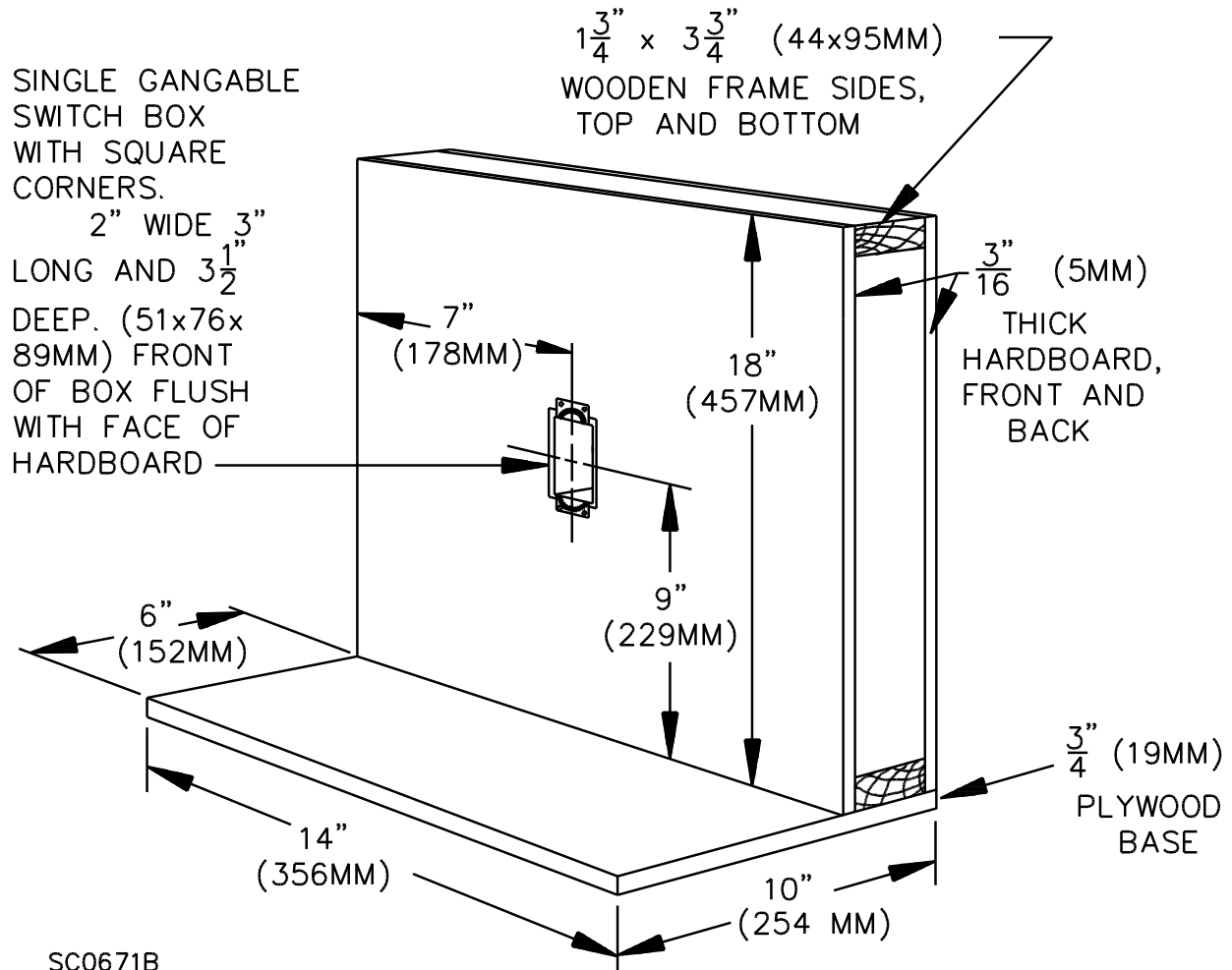
Figure 140.1 Test frame
