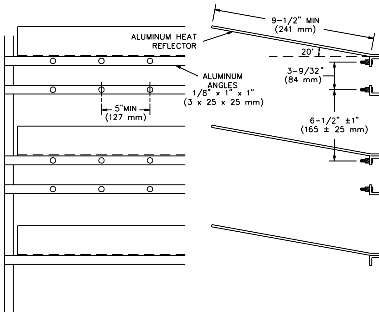
Figure 137.2 Test fixture
