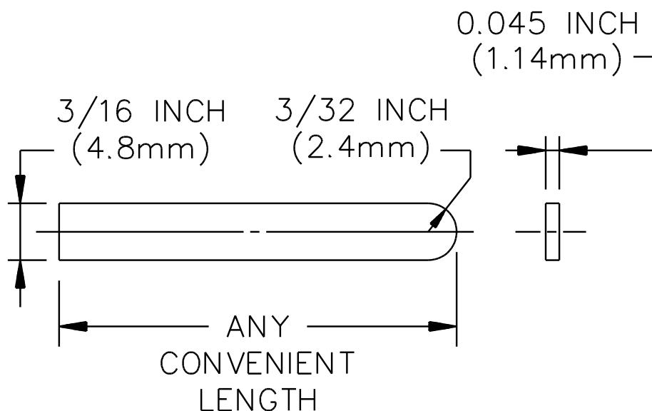
Figure 31.1 Flat probe
