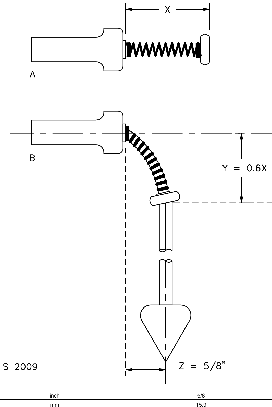
Figure 191.1 Test of cord guard
