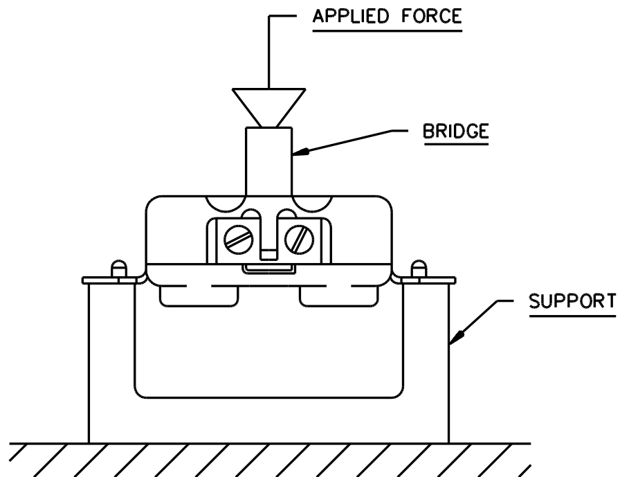
Figure 124.4 Assembly security test method (inverted)
