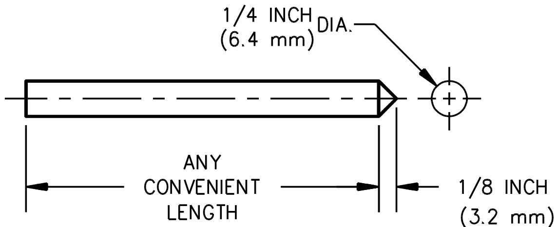
Figure 10.1 Probe
