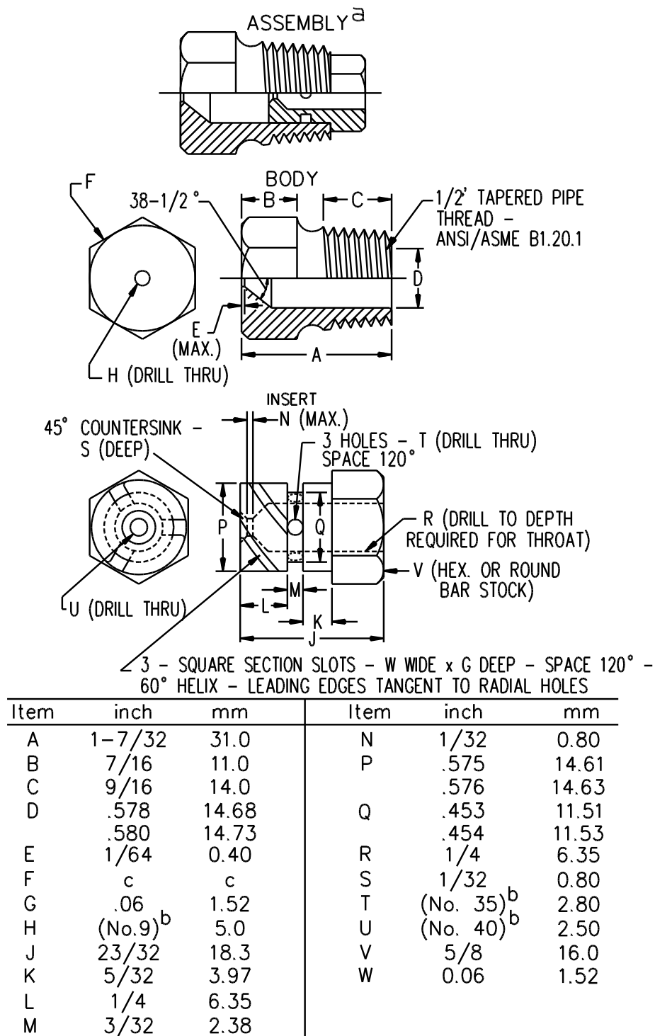
Figure SB11.2 Water-spray head
